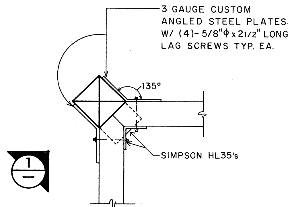
FRAMING DETAIL
