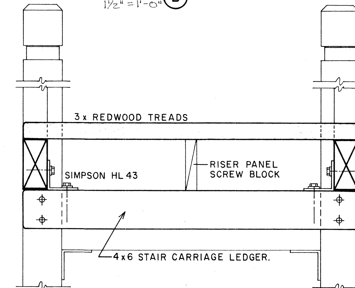
TRANSVERSE STAIR SECTION
