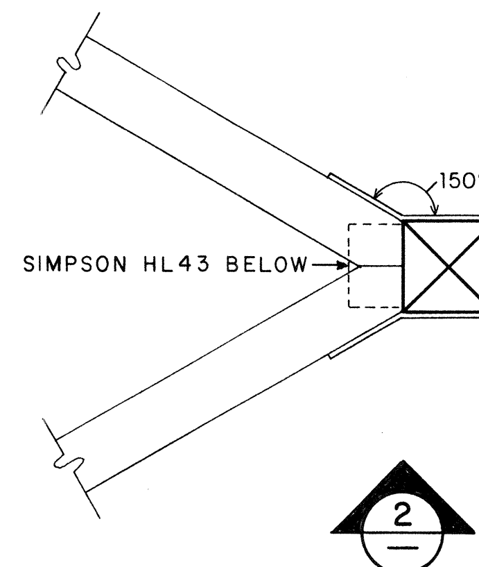
FRAMING DETAIL
