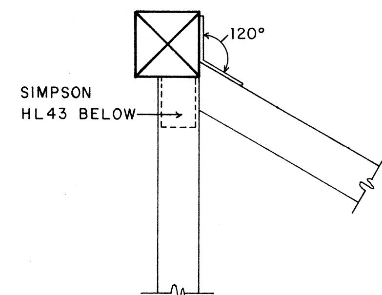
FRAMING DETAIL
