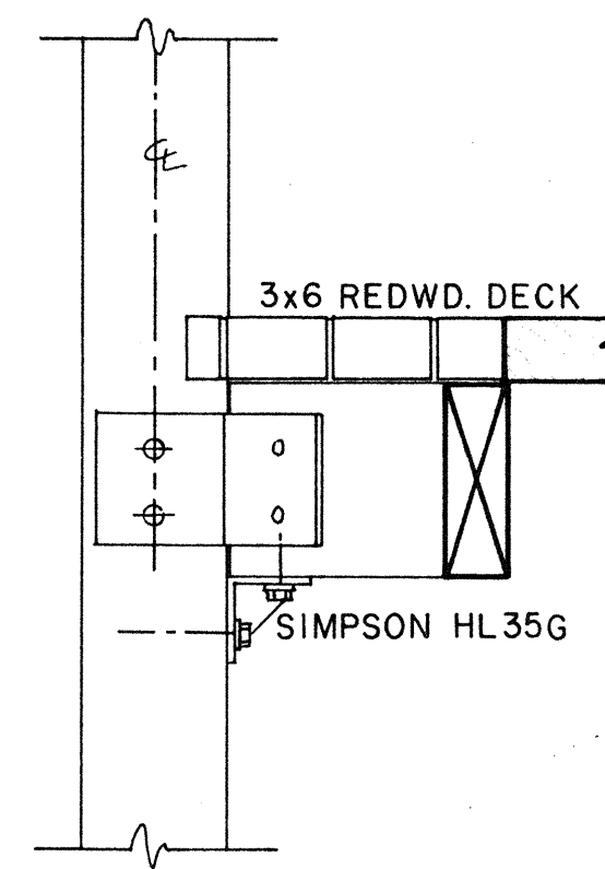
ELEVATION DETAIL
