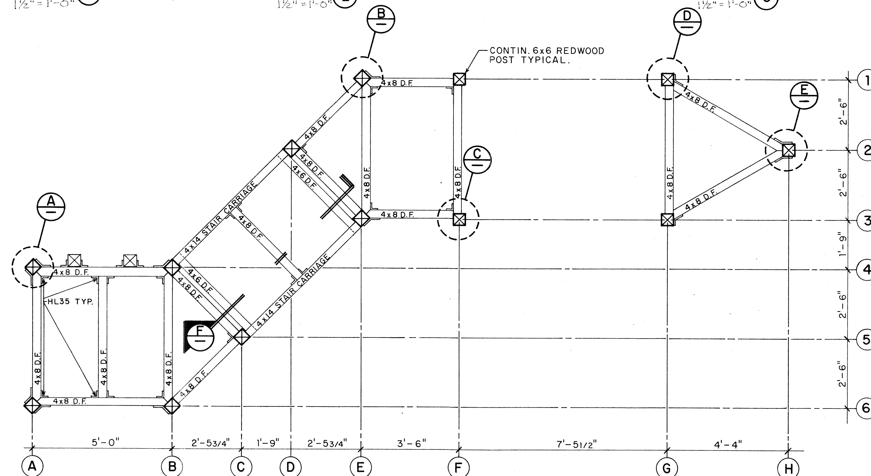
STRUCTURE "C" DECK FRAMING PLAN
