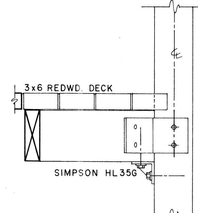
ELEVATION DETAIL
