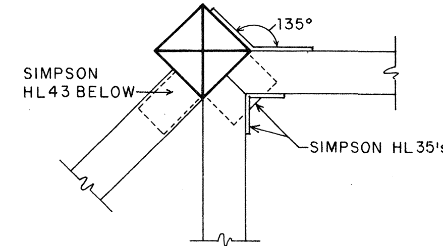
FRAMING DETAIL
